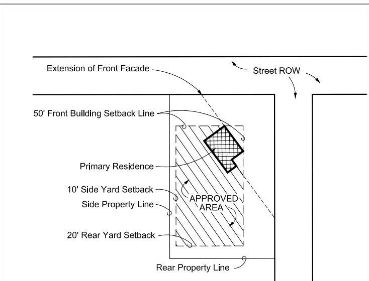
Standard corner lot with angled house layout
