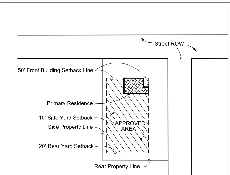
Standard Corner Lot
